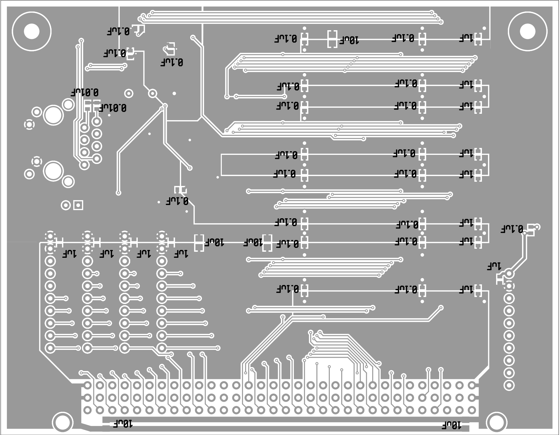
layer bottomassembly
